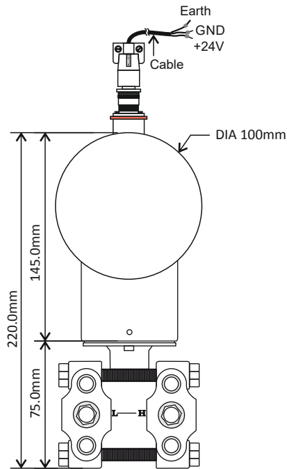
Fig.1 Front View
