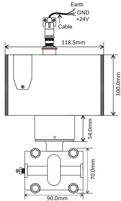
Fig.2 Side View
