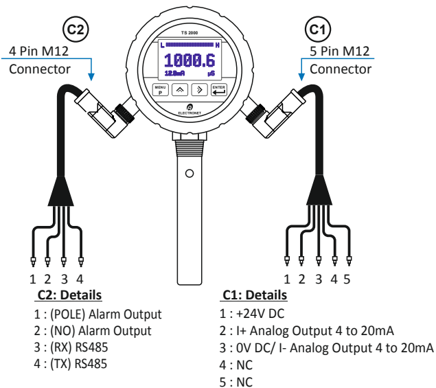
Fig. 3 Front View
