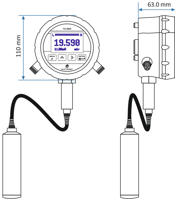
Fig. 1 Front View
