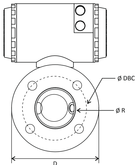
Fig. 2 Side View
