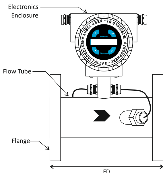
Fig. 1 Front View
