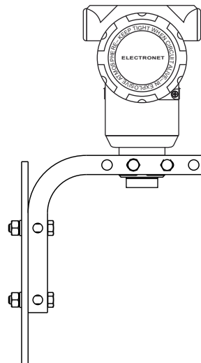
Panel Mounting
