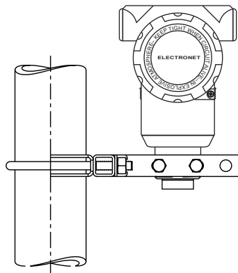
Pipe Mounting
